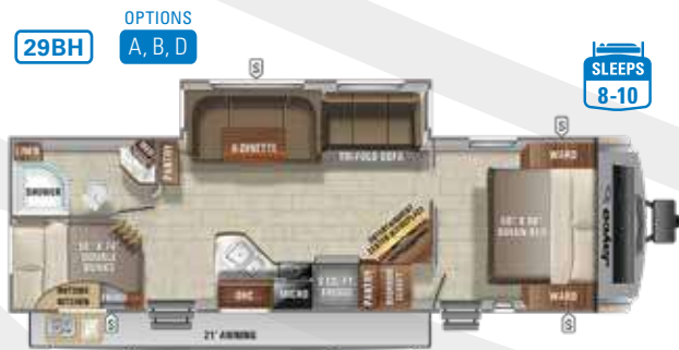
Ext. Lgth: 34' 9" Weight: 7,180 lbs. Hitch: 830 lbs.
