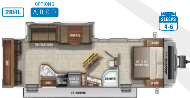
Ext. Lgth: 33' 6" Weight: 6,805 lbs. Hitch: 785 lbs.
