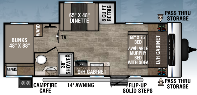
SN211VDB | 4,620 UVW | 27' LENGTH | SLEEPS 8
