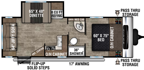
SN231VRL | 4,480 UVW | 26' 11" LENGTH | SLEEPS 6
