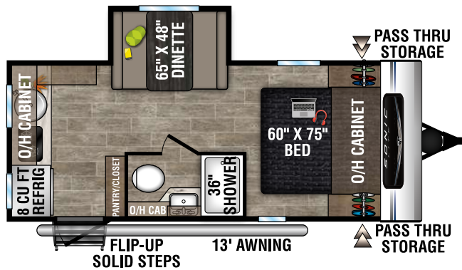
SLI69VRK | 3,570 UVW | 22' 1" LENGTH | SLEEPS 4
