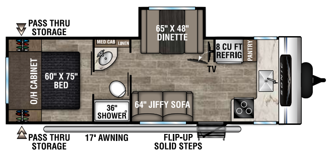
SN241VFK | 4,520 UVW | 28' 4" LENGTH | SLEEPS 4 NEW
