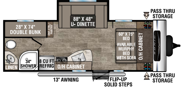
SN220VBH | 4,480 UVW | 26' 7" LENGTH | SLEEPS 6
