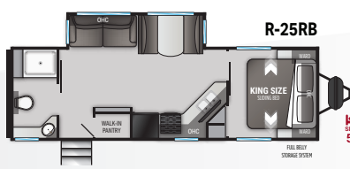
Length 30' 8" Dry 6,080 lbs. Hitch 780 lbs. Height 11' 3"
