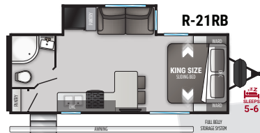
Length 25' 11" Dry 5,346 lbs. Hitch 702 lbs. Height 11' 1"
