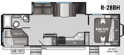
Length 32' 11" Dry 6,938 lbs. Hitch 1,108 lbs. Height 11' 3"
