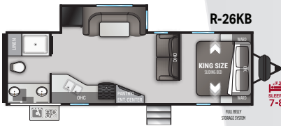
Length 30' 11" Dry 5,856 lbs. Hitch 644 lbs. Height 11' 1"
