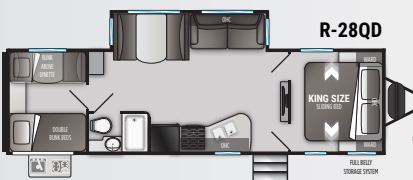
Length 33' 4" Dry 6,404 lbs. Hitch 800 lbs. Height 11' 3"
