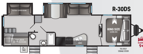
Length 36' 5" Dry 7,160 lbs. Hitch 940 lbs. Height 11' 5"
