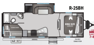
Length 29' 11" Dry 5,727 lbs. Hitch 736 lbs. Height 11' 1"
