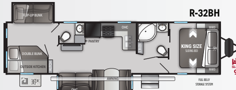
Length 36' 7" Dry 7,532 lbs. Hitch 1,042 lbs. Height 11' 5"
