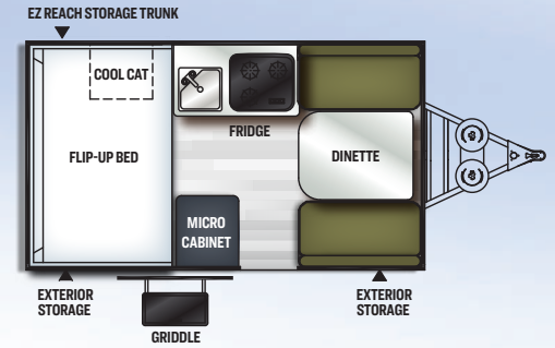
T12RB HARD SIDE FLAGSTAFF UVW: 2014 CCC: 1208 AXLE: 1754 HITCH: 222 CLOSED HEIGHT: 5' 1" CLOSED LENGTH W/ HITCH: 17' 5" BOX SIZE: 12' FRESH: 20 GRAY: N/A BLACK: N/A
