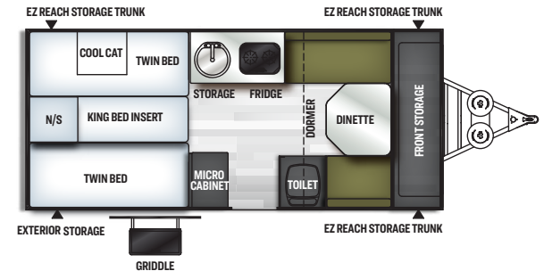
T21TBHW HARD SIDE FLAGSTAFF UVW: 2670 CCC: 702 AXLE: 2260 HITCH: 372 CLOSED HEIGHT: 5' 8" CLOSED LENGTH W/ HITCH: 21' 2" BOX SIZE: 14' FRESH: 20 GRAY: N/A BLACK: N/A
