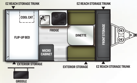
T12RBST HARD SIDE FLAGSTAFF UVW: 2120 CCC: 1164 AXLE: 1798 HITCH: 284 CLOSED HEIGHT: 5' 1" CLOSED LENGTH W/ HITCH: 19' 2" BOX SIZE: 12' FRESH: 20 GRAY: N/A BLACK: N/A
