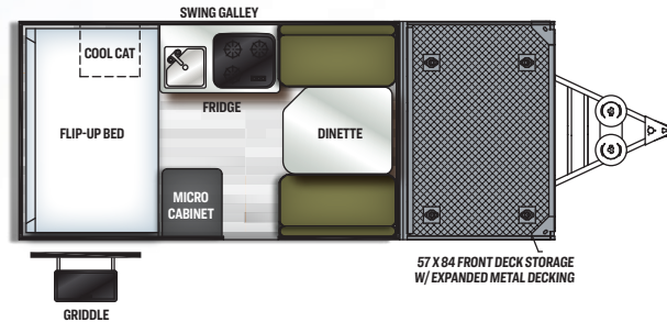
T12RBTH HARD SIDE FLAGSTAFF UVW: 2408 CCC: 1387 AXLE: 2075 HITCH: 295 CLOSED HEIGHT: 5' 8" CLOSED LENGTH W/ HITCH: 22' 3" BOX SIZE: 12' FRESH: 20 GRAY: N/A BLACK: N/A
