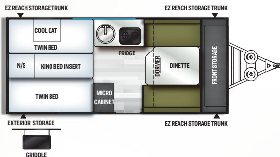
T21BHWOR HARD SIDE FLAGSTAFF UVW: 2698 CCC: 1107 AXLE: 2355 HITCH: 305 CLOSED HEIGHT: 6' 1" CLOSED LENGTH W/ HITCH: 21' 2" BOX SIZE: 14' FRESH: 20 GRAY: N/A BLACK: N/A
