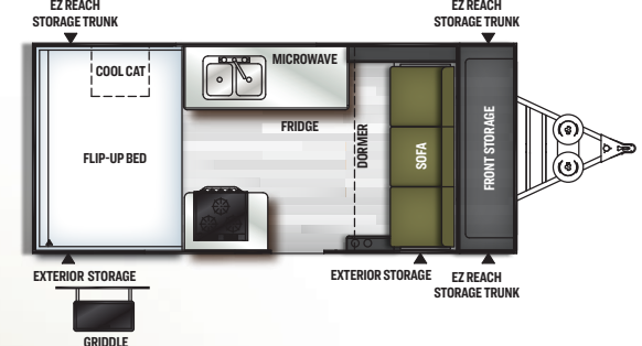
T21FSHW HARD SIDE FLAGSTAFF UVW: 2648 CCC: 667 AXLE: 2295 HITCH: 315 CLOSED HEIGHT: 5' 8" CLOSED LENGTH W/ HITCH: 21' 2" BOX SIZE: 14' FRESH: 20 GRAY: N/A BLACK: N/A
