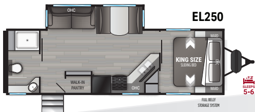
Length 30' 8" Dry 6,080 lbs. Hitch 780 lbs. Height 11' 3"
