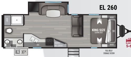
Length 30' 11" Dry 5,904 lbs. Hitch 656 lbs. Height 11' 1"
