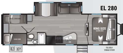
Length 33' 4" Dry 6,360 lbs. Hitch 820 lbs. Height 11' 3"
