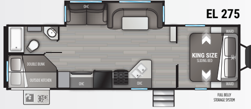
Length 32' 11" Dry 6,300 lbs. Hitch 680 lbs. Height 11' 3"
