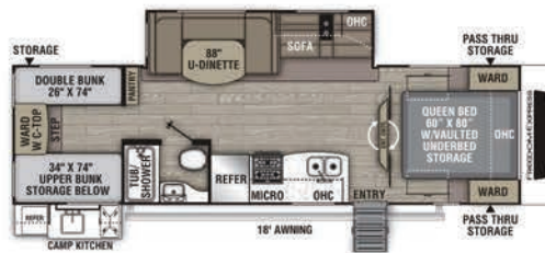
292 BHDS / Exterior Length 33' 4"
